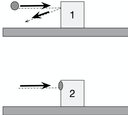
Figure 2. Two balls of equal mass are thrown horizontally with the same initial velocity. They hit identical stationary boxes resting on a frictionless horizontal surface. The ball hitting box 1 bounces back, while the ball hitting box 2 gets stuck. Which box ends up moving faster? Figure adapted from Gladding, et al (2014).
