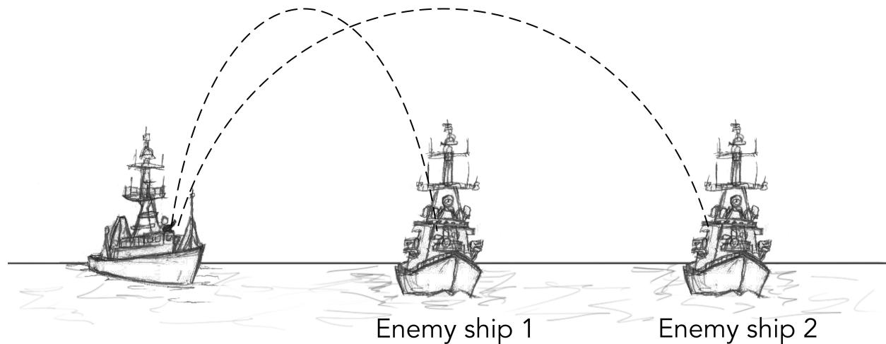
Figure 1. “Which ship gets hit first?” Figure adapted from Gladding, et al (2014). Sketch by Benjamin Hammer
