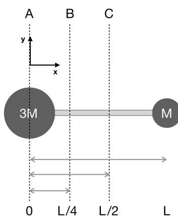
Figure 3. A ball of mass 3M at x=0 is connected to a ball of mass M at x=L by a massless rod. Consider the three rotation axes A, B and C as shown, all parallel to the y -axis. For which rotation axis is the moment of inertia of the object smallest? (It may help you to figure out where the center of mass of the object is.) Figure adapted from Gladding, et al (2014).
